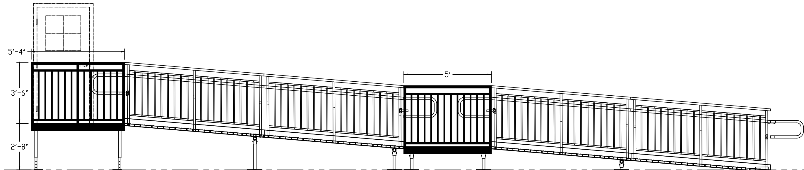
ELEV VIEW: 42/34 VP ALUMINUM ACCESS RAMP SYSTEM NOTE: CAN BE ASSEMBLED WITH OTHER RAMP SIZES
