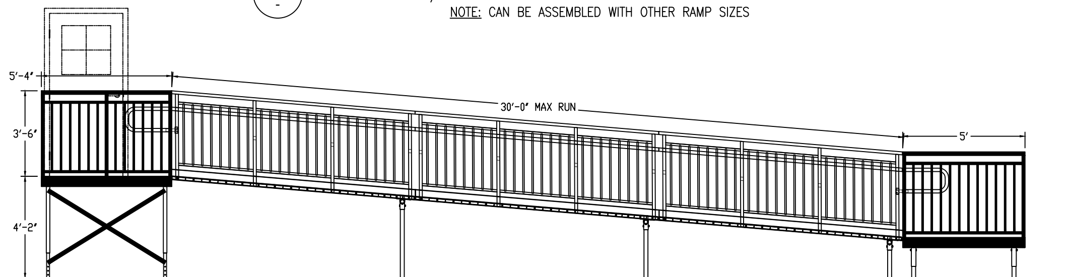
B-B ELEV VIEW: 42/34 VP ALUMINUM ACCESS RAMP SYSTEM NOTE: CAN BE ASSEMBLED WITH OTHER RAMP SIZES
