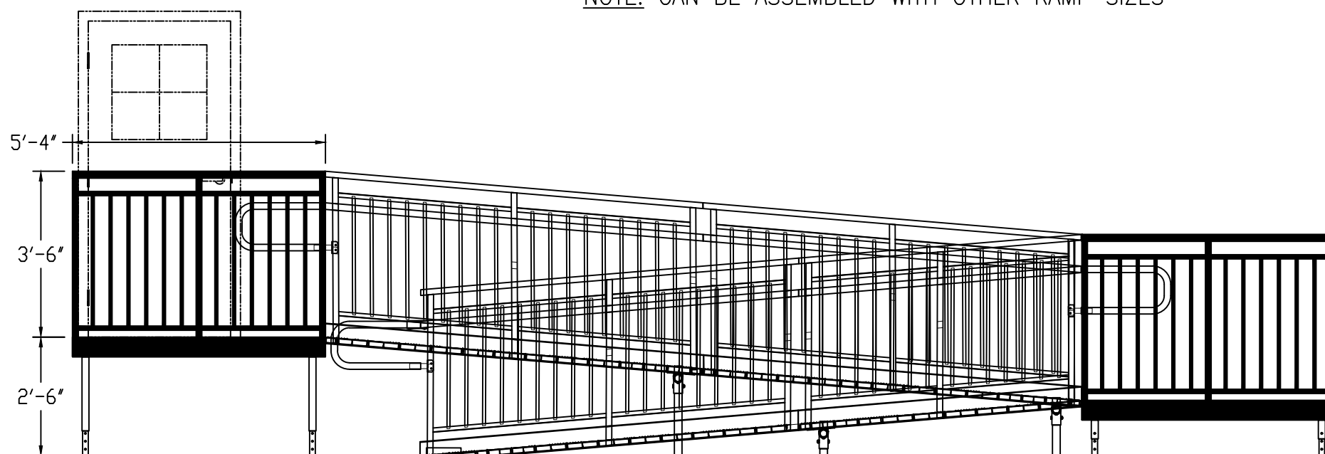
ELEV VIEW: 42/34 VP ALUMINUM ACCESS RAMP SYSTEM
