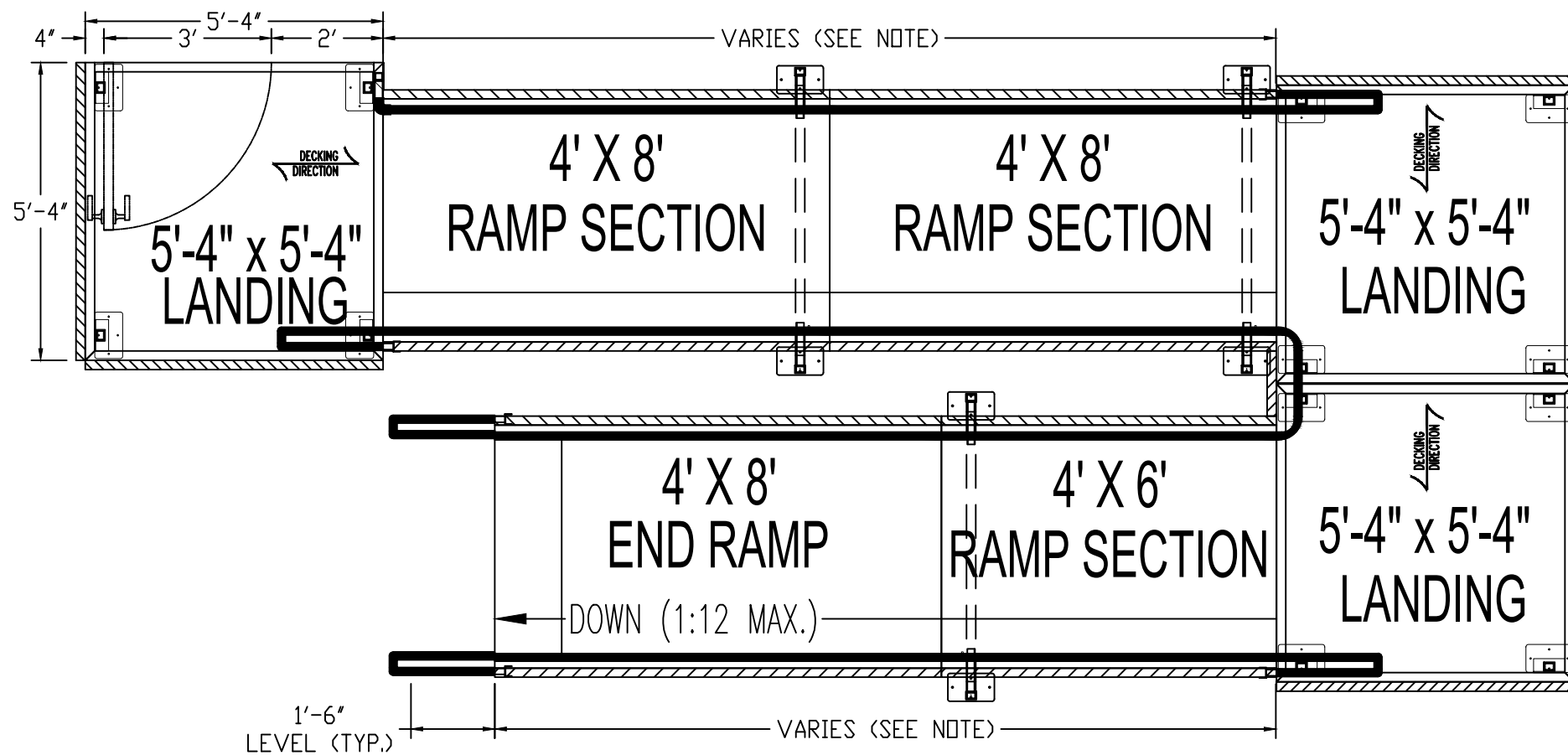
PLAN VIEW: 42/34 VP ALUMINUM ACCESS RAMP SYSTEM
