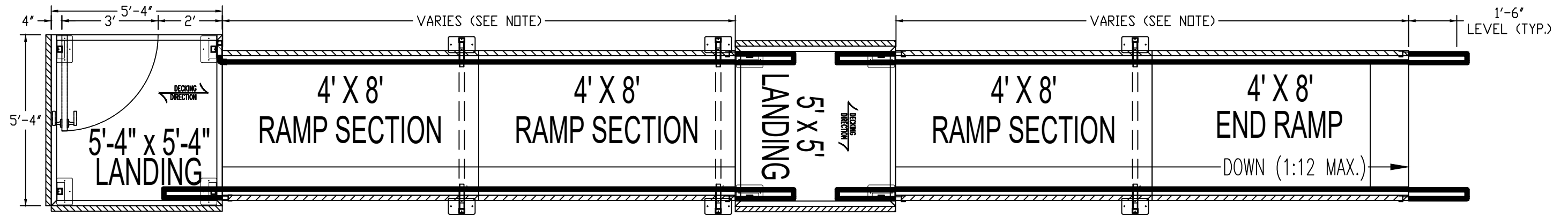
PLAN VIEW: 42/34 VP ALUMINUM ACCESS RAMP SYSTEM NOTE: CAN BE ASSEMBLED WITH OTHER RAMP SIZES
