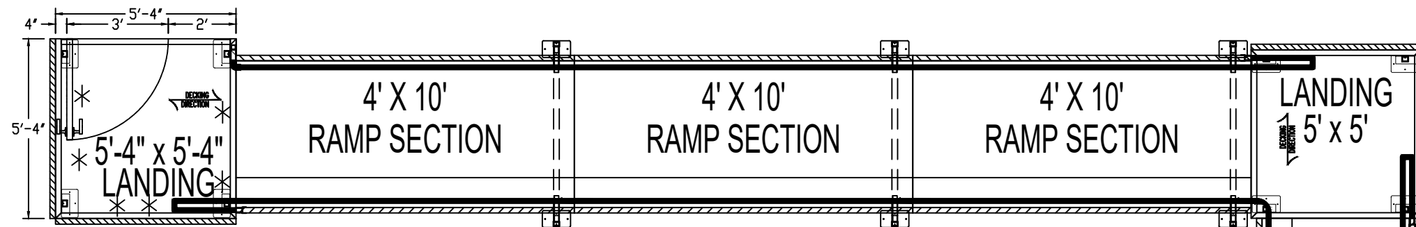
PLAN VIEW: 42/34 VP ALUMINUM ACCESS RAMP SYSTEM NOTE: CAN BE ASSEMBLED WITH OTHER RAMP SIZES
