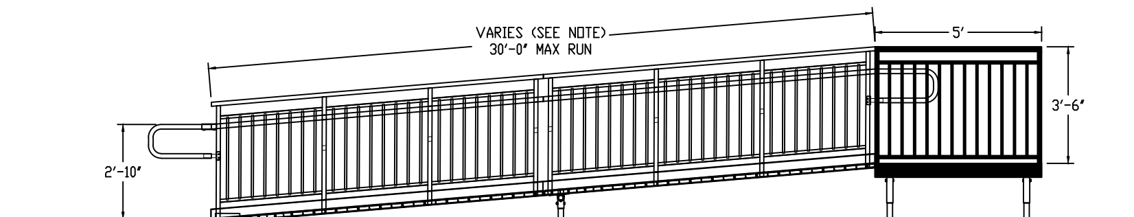
C-C ELEV VIEW: 42/34 VP ALUMINUM ACCESS RAMP SYSTEM NOTE: CAN BE ASSEMBLED WITH OTHER RAMP SIZES
