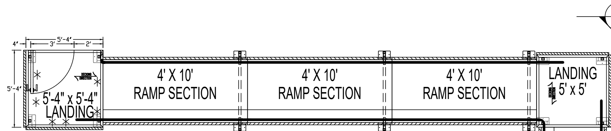
PLAN VIEW: 42/34/23 VP ALUMINUM ACCESS RAMP SYSTEM NOTE: CAN BE ASSEMBLED WITH OTHER RAMP SIZES
