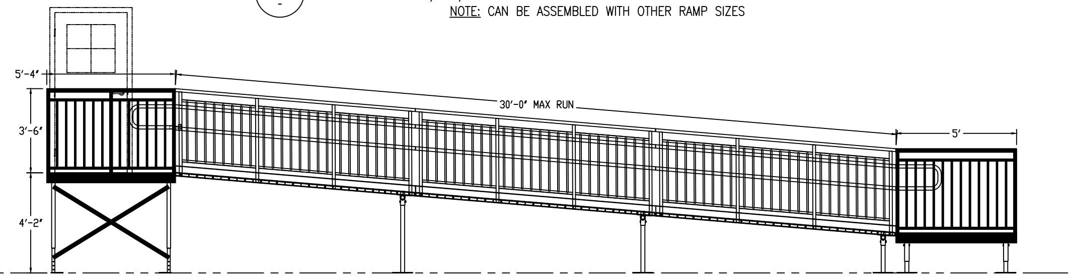
B-B ELEV VIEW: 42/34/23 VP ALUMINUM ACCESS RAMP SYSTEM NOTE: CAN BE ASSEMBLED WITH OTHER RAMP SIZES
