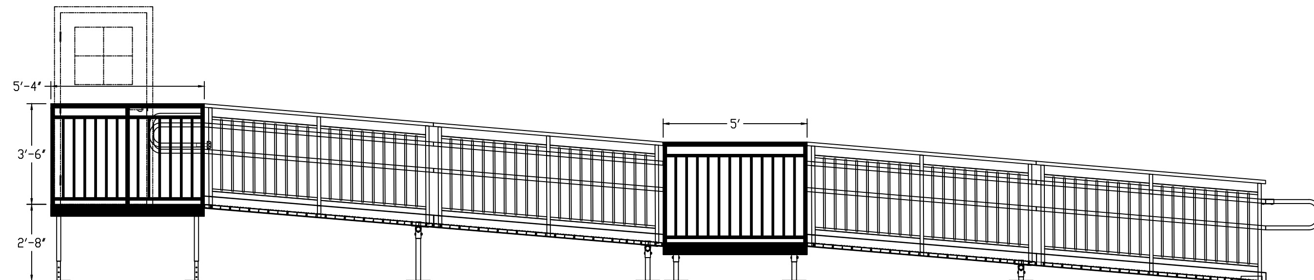
ELEV VIEW: 42/34/23 VP ALUMINUM ACCESS RAMP SYSTEM NOTE: CAN BE ASSEMBLED WITH OTHER RAMP SIZES
