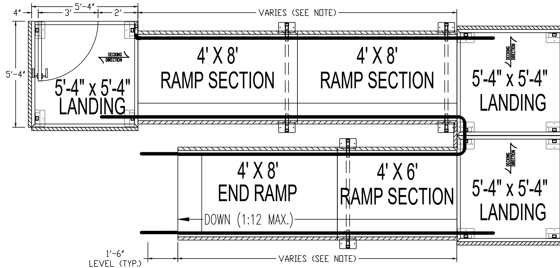
PLAN VIEW: 42/34/23 VP ALUMINUM ACCESS RAMP SYSTEM
