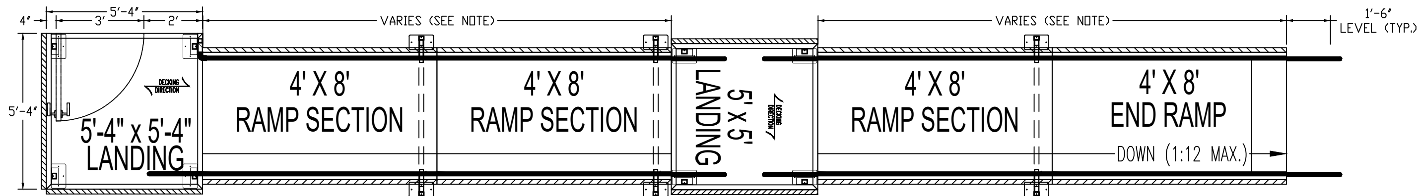
PLAN VIEW: 42/34/23 VP ALUMINUM ACCESS RAMP SYSTEM NOTE: CAN BE ASSEMBLED WITH OTHER RAMP SIZES
