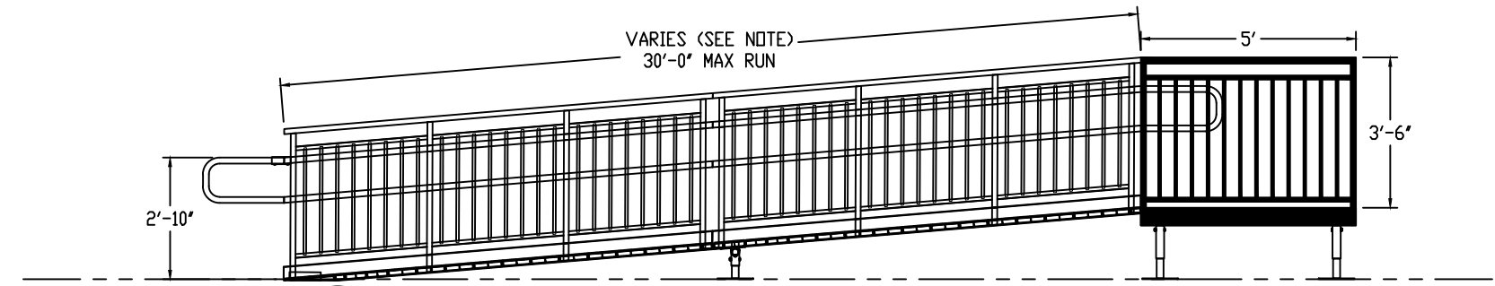
C-C ELEV VIEW: 42/34/23 VP ALUMINUM ACCESS RAMP SYSTEM NOTE: CAN BE ASSEMBLED WITH OTHER RAMP SIZES
