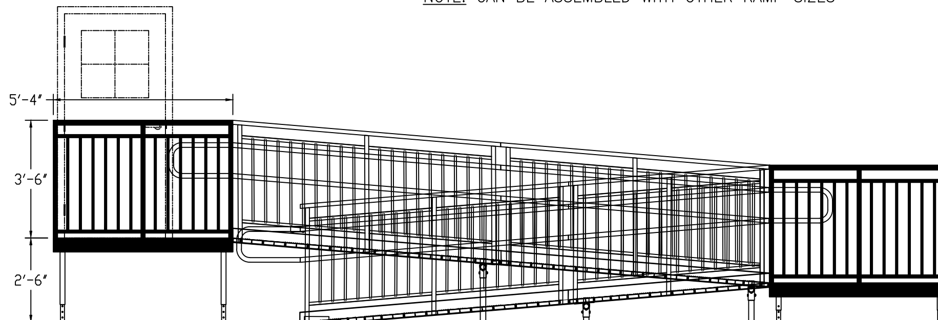
ELEV VIEW: 42/34/23 VP ALUMINUM ACCESS RAMP SYSTEM
