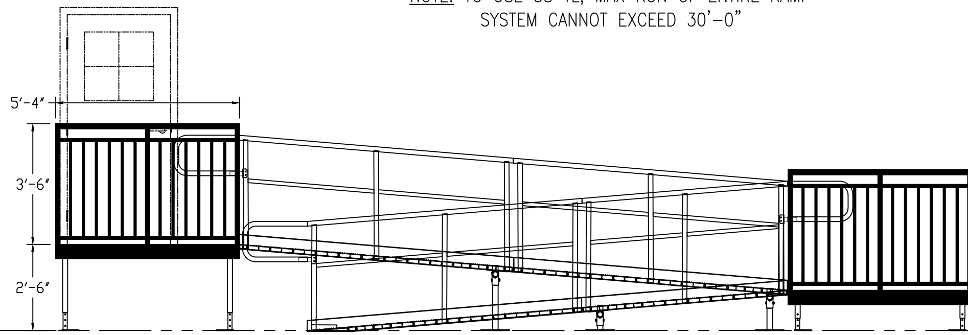
ELEV VIEW: 38 TWO LINE ALUMINUM ACCESS RAMP SYSTEM NOTE: TO USE 38 TL, MAX RUN OF ENTIRE RAMP SYSTEM CANNOT EXCEED 30'-0"
