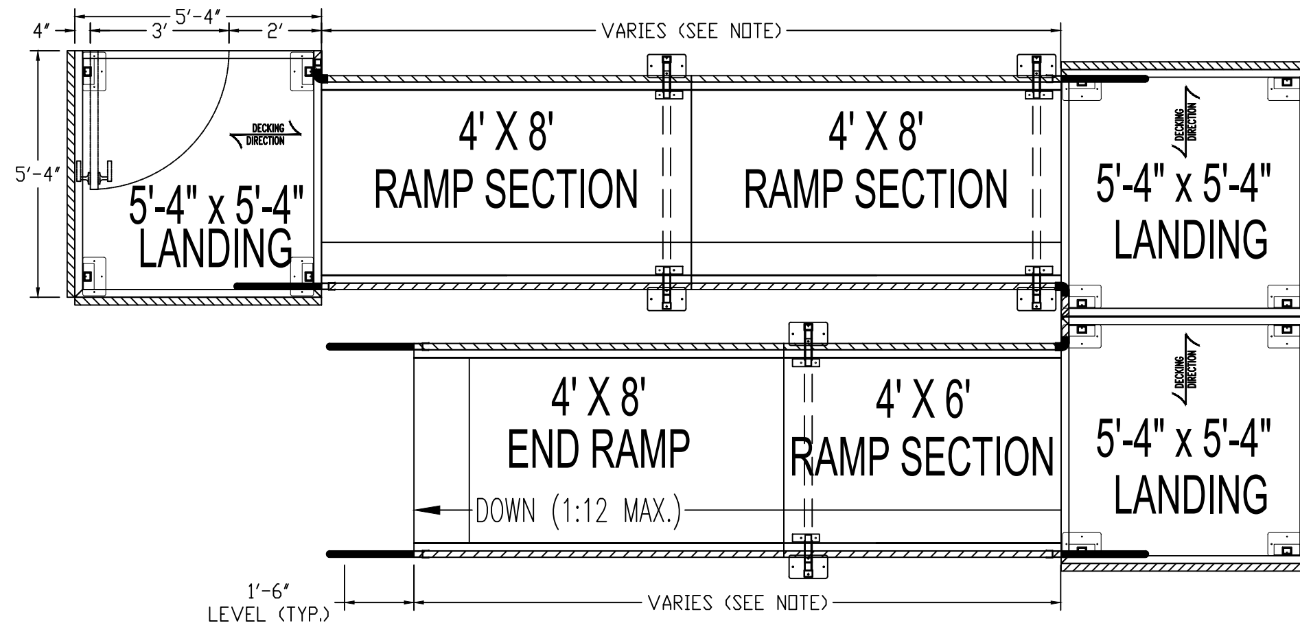
PLAN VIEW: 38 TWO LINE ALUMINUM ACCESS RAMP SYSTEM NOTE: TO USE 38 TL, MAX RUN OF ENTIRE RAMP SYSTEM CANNOT EXCEED 30'-0"
