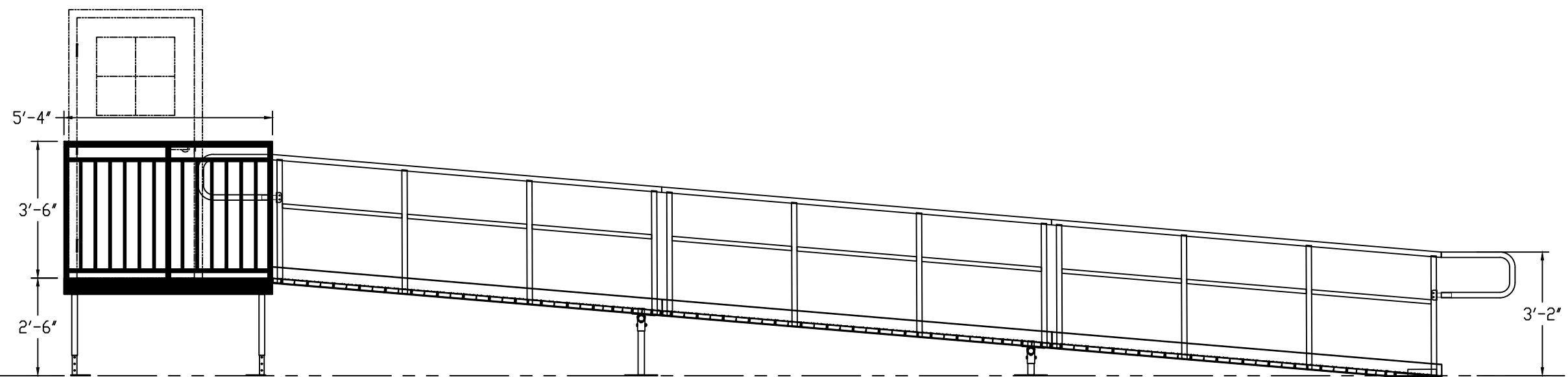
ELEV VIEW: 38 TWO LINE ALUMINUM ACCESS RAMP SYSTEM
