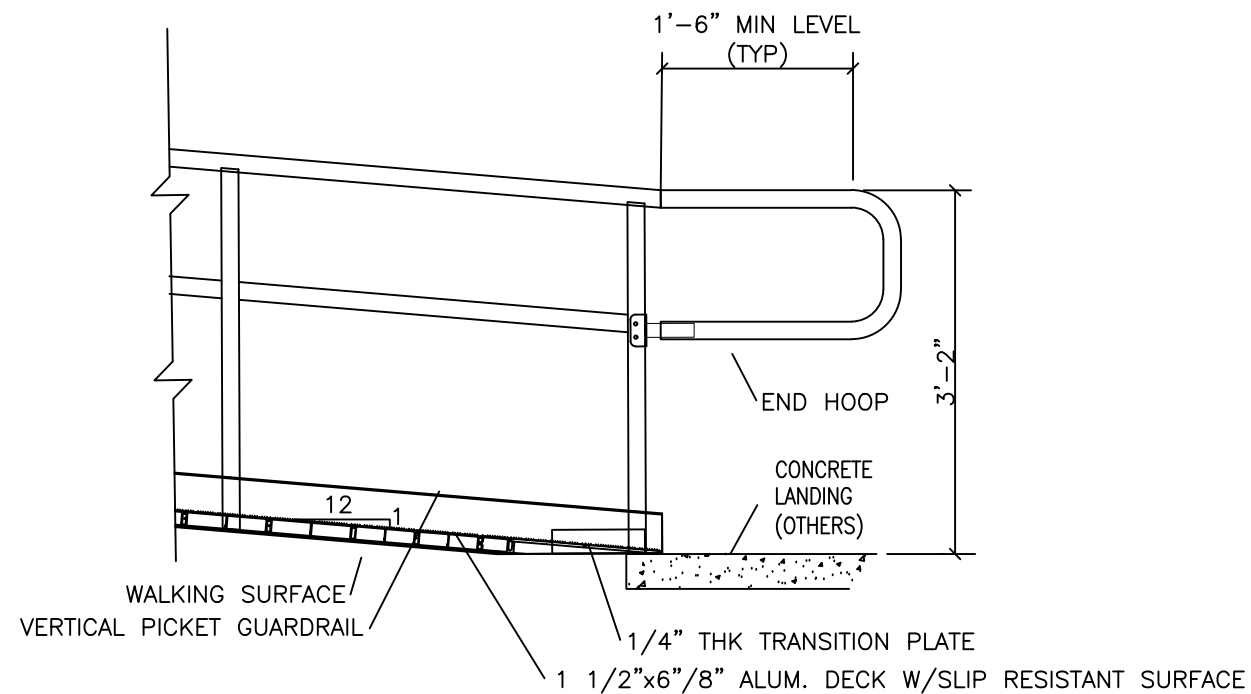
DETAIL END RAMP (1:12 SLOPE)
