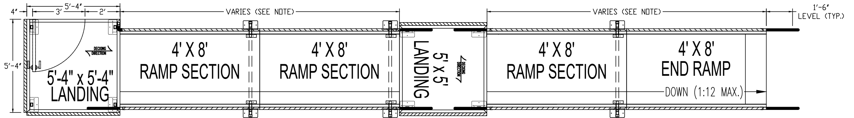
PLAN VIEW: 38 TWO LINE ALUMINUM ACCESS RAMP SYSTEM
