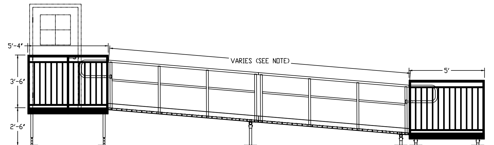
ELEV VIEW: 38 TWO LINE ALUMINUM ACCESS RAMP SYSTEM NOTE: TO USE 38 TL, MAX RUN OF ENTIRE RAMP SYSTEM CANNOT EXCEED 30'-0"
